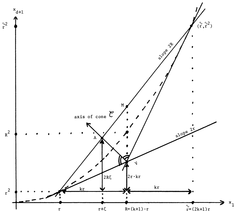
FIGURE. Paraboloid \mathcal{P} of revolution and tangential cone \mathcal{C} intersected with x_1 - x_{d+1} -plane. The “axis” is the angle bisector of the two generators of the cone \mathcal{C} in this plane.
